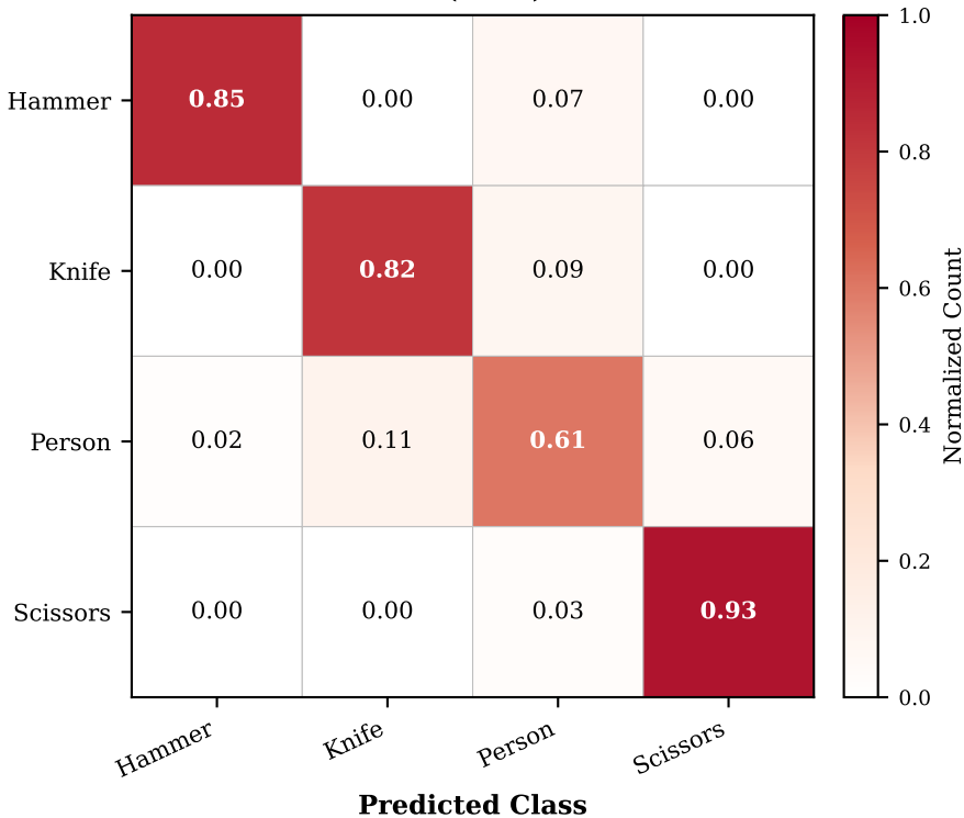
Confusion Matrix (Normalized) Fine-tuned v5 (Final) --- Test Set
